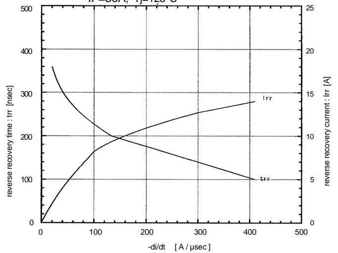
Reverse recovery time characteristics vs. -di/dt IF=30A, Tj=125°C
