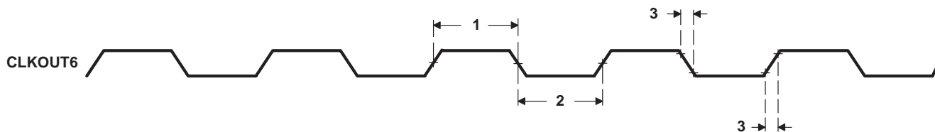
Figure 4-7. CLKOUT6 Timing
