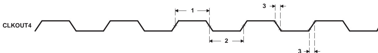
Figure 4-6. CLKOUT4 Timing
