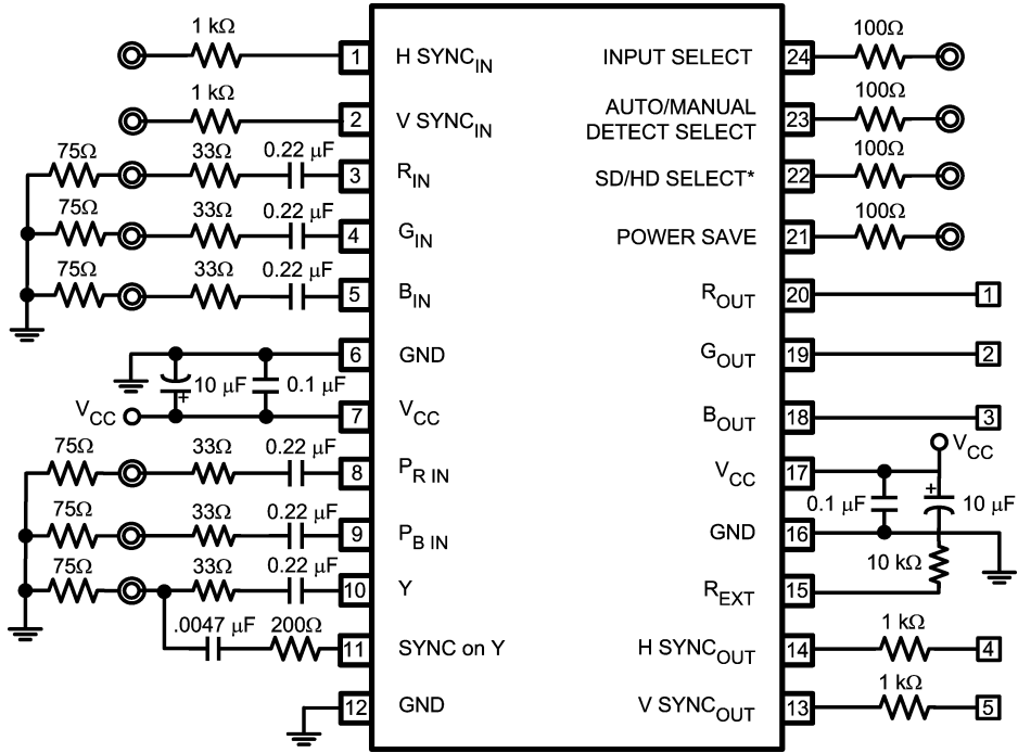
FIGURE 3. Test Circuit
