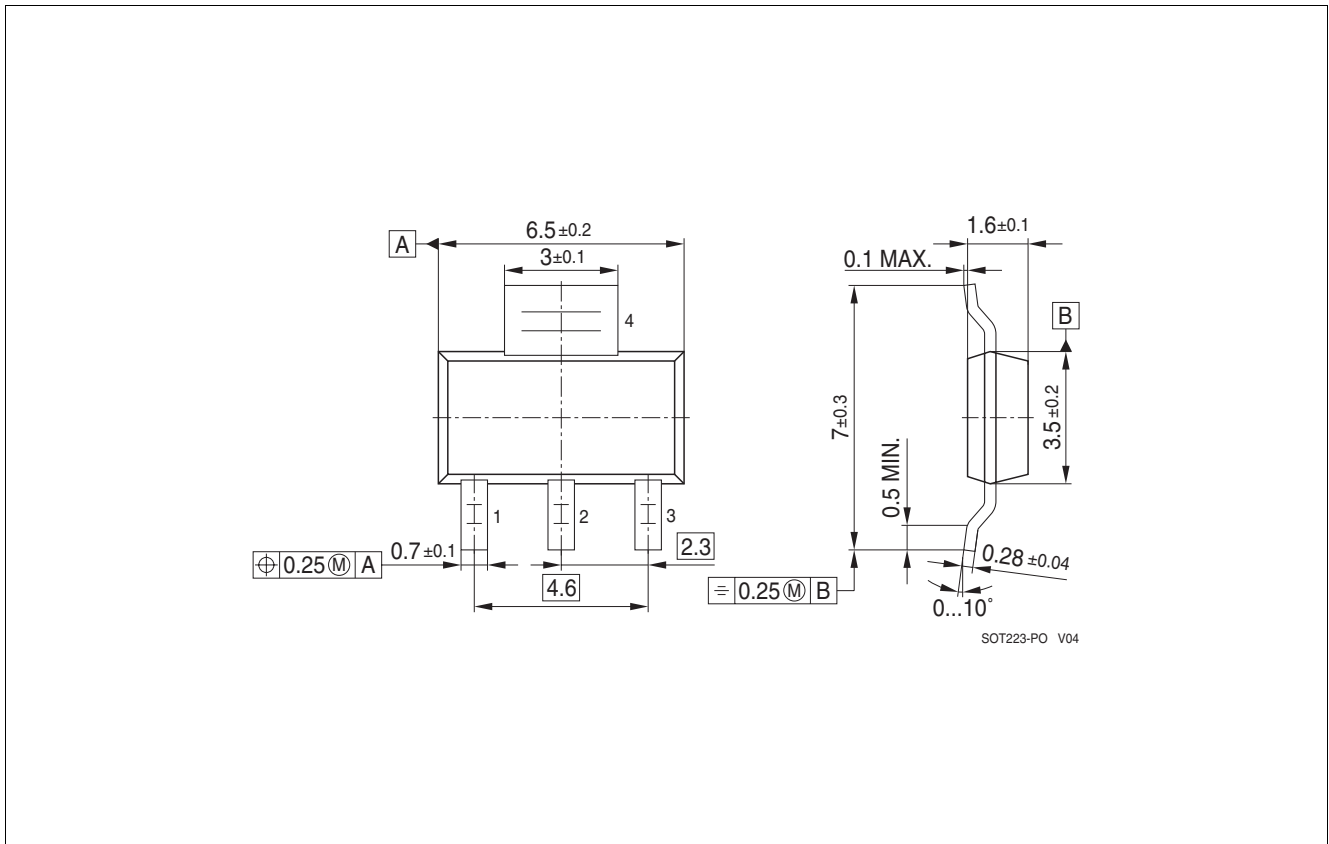
Figure 7 PG-SOT223-4
