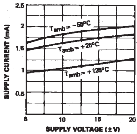
SUPPLY CURRENT
