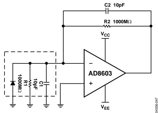
Figure 47. Photodiode Circuit
