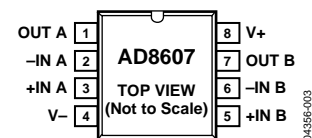
Figure 3. 8-Lead SOIC_N (R Suffix)
