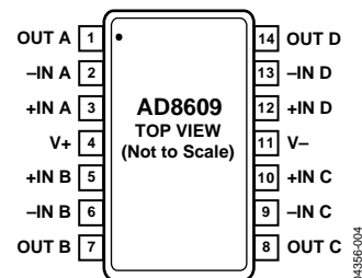
Figure 4. 14-Lead TSSOP (RU Suffix)
