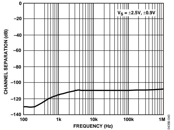
Figure 40. Channel Separation
