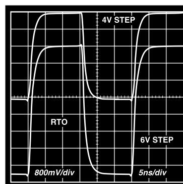
Figure 10.* Step Response; G = -2, V S = ±5 V
