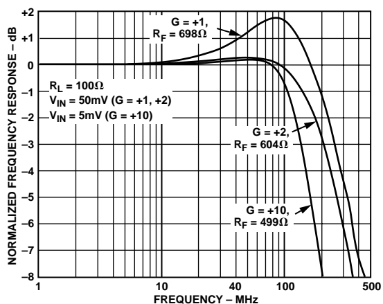
Figure 7. Frequency Response; G = +1, +2, +10, V S = ±5 V
