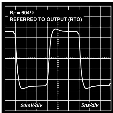
Figure 5.* 100 mV Step Response; G = +2, V S = ±2.5 V or ±5 V
