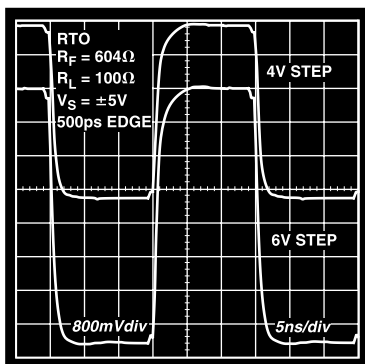
Figure 6.* Step Response; G = +2, V S = ±5 V
