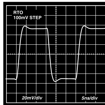
Figure 9.* 100 mV Step Response; G = -2, V S = ±2.5 V or ±5 V
