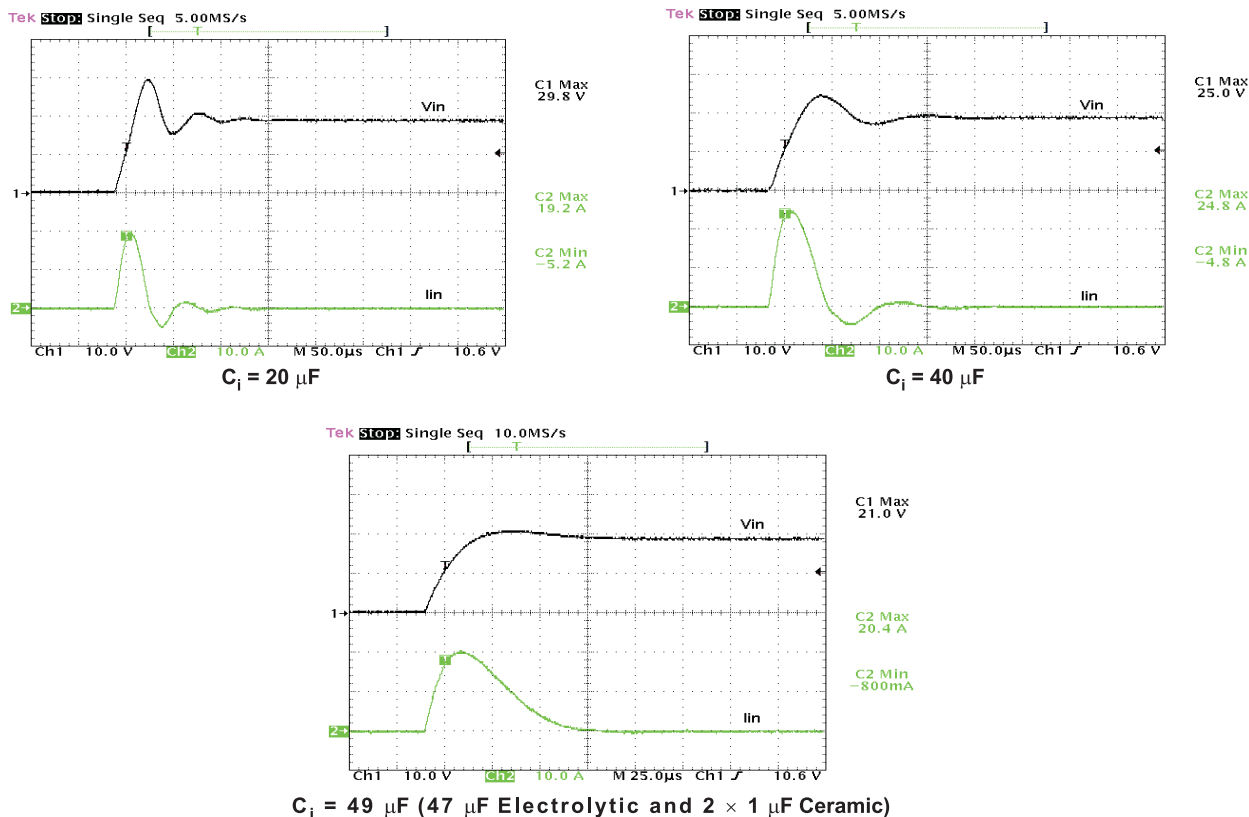
Figure 31. Adapter DC Side Hot Plug-In With Various Input Capacitances
