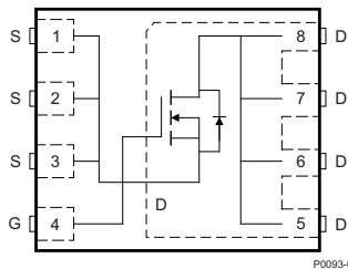
Figure 1. Top View
