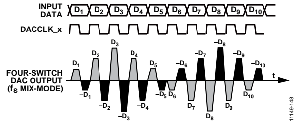
Figure 145. Mix-Mode Waveform
