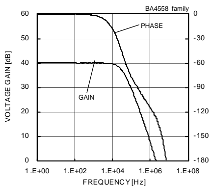
Fig.22 Voltage Gain - Frequency ( V_{CC}/V_{EE}=+15[V]/-15[V] , A_v=40[dB] , R_L=2[k\Omega] , T_a=25[^\circ C] )
