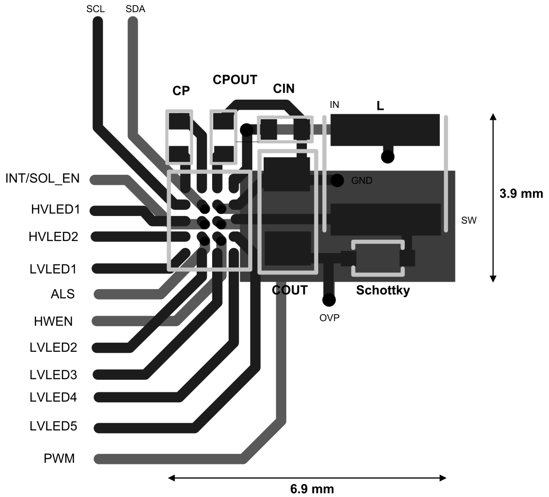
FIGURE 20. LM3533 Example Layout
