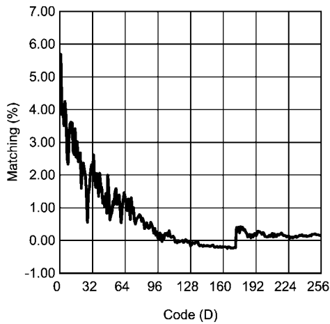
HVLED Matching vs Code (VIN = 3.6V, Exponential Mode)
