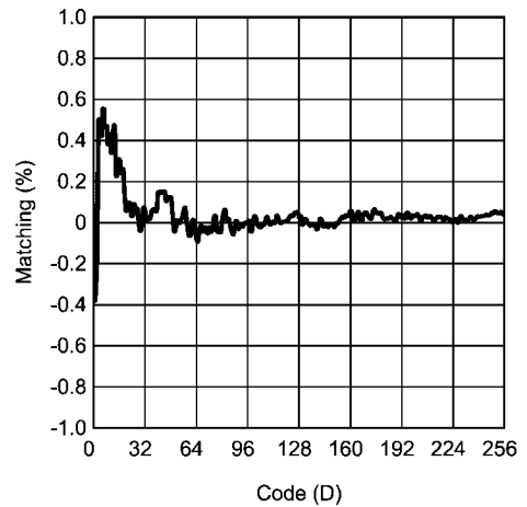
HVLED Matching vs Code (VIN = 3.6V, Linear Mode)
