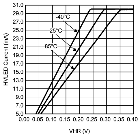
HVLED Current vs Current Sink Headroom Voltage
