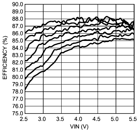
Efficiency vs VIN, Single String L = 10 \mu H, 20mA/string, f SW = 500kHz Top to Bottom: 1x4, 1x5, 1x6, 1x7, 1x8, 1x9, 1x10 (LEDs)
