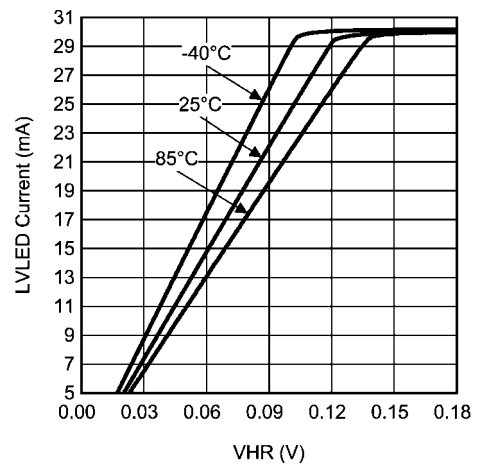
LVLED Current vs Current Sink Headroom Voltage
