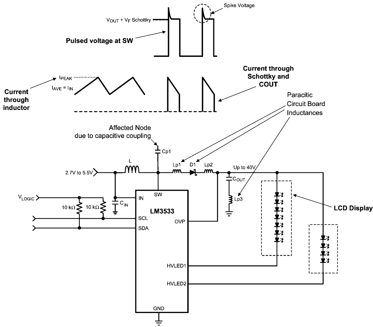
FIGURE 18. LM3533's Inductive Boost Converter Showing Pulsed Voltage at SW (High dV/dt) and Current Through Schottky and COUT (High di/dt)
