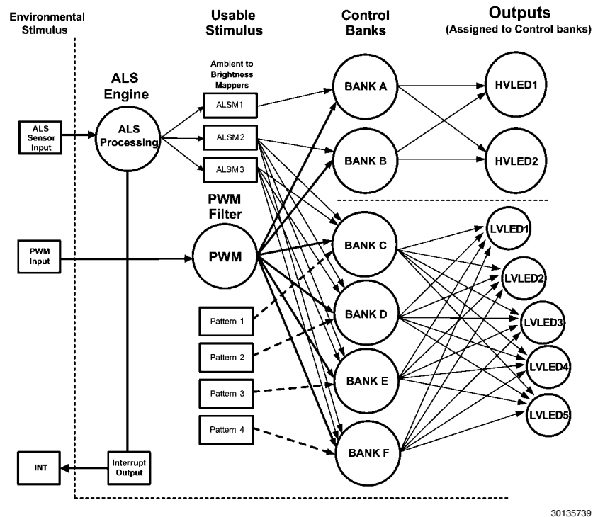
FIGURE 3. Functional Control Diagram
