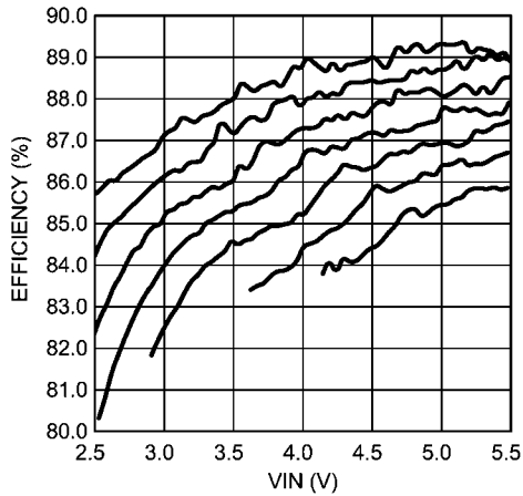
Efficiency vs VIN, Dual String L = 10 \mu H, 20mA/string, f SW = 500kHz Top to Bottom: 2x4, 2x5, 2x6, 2x7, 2x8, 2x9, 2x10 (LEDs)
