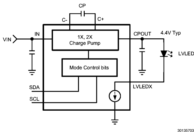
FIGURE 4. Integrated Charge Pump
