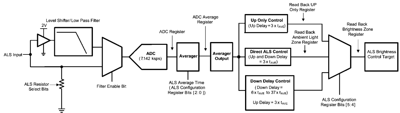
FIGURE 8. Ambient Light Sensing Block Diagram
