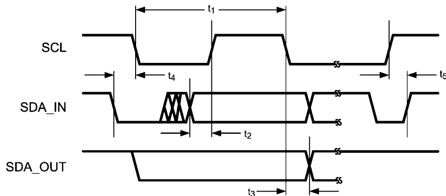
FIGURE 1. I 2 C-Compatible Interface Timing
