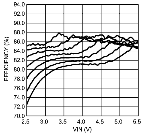
Efficiency vs VIN, Single String L = 10 \mu H, 20mA/string, f SW = 1MHz Top to Bottom: 1x4, 1x5, 1x6, 1x7, 1x8, 1x9, 1x10 (LEDs)
