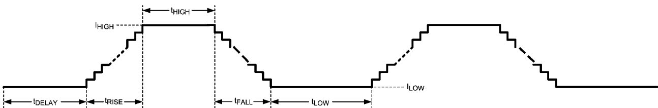
FIGURE 14. Pattern Generator Timing
