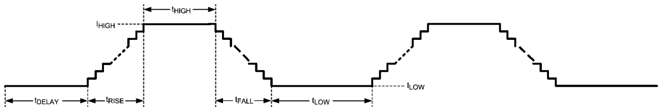
FIGURE 17. Pattern Generator Timing
