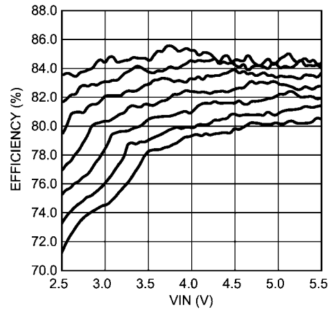
Efficiency vs VIN, Single String L = 4.7 \mu H, 20mA/string Top to Bottom: 1x4, 1x5, 1x6, 1x7, 1x8, 1x9, 1x10 (LEDs)
