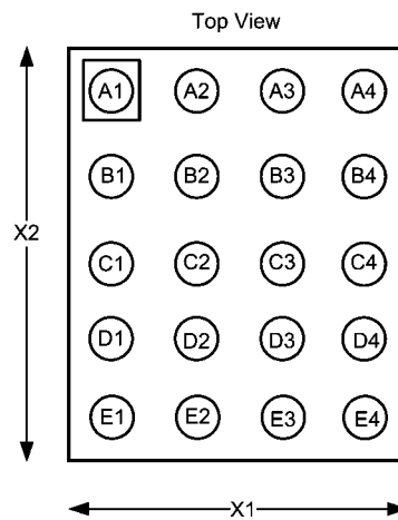
30135702 20-Bump micro SMD Package TMD20GAA (X1 = 1.755mm ( \pm 30 \mu m), X2 = 2.015mm ( \pm 30 \mu m))
