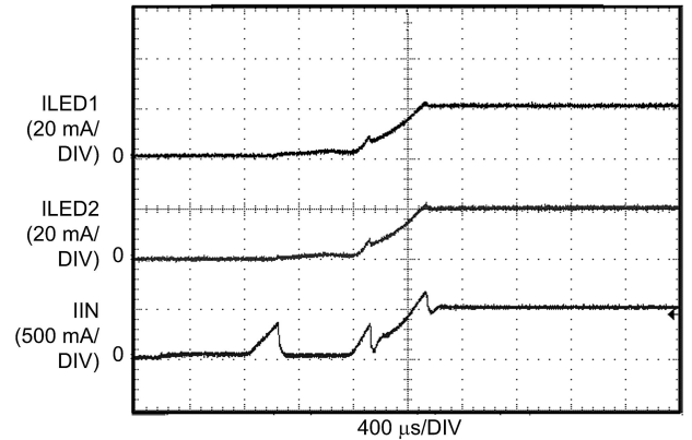
Startup Response (VIN = 3.6V, 2x8 LEDs, 20mA/string)
