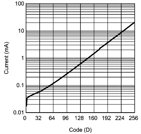
HVLED Current vs Code (VIN = 3.6V, Exponential Mode)
