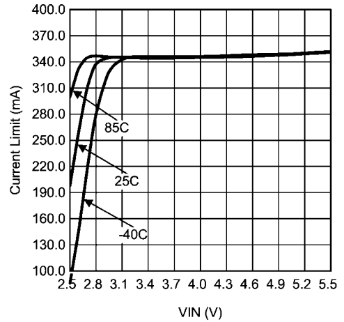
Charge Pump Short Circuit Current Limit vs VIN (1X Gain)
