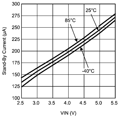
Idle State Supply Current (Pattern Generator Enabled on LVLED1, LVLED2, LVLED3)
