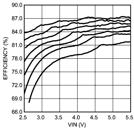
Efficiency vs VIN, Dual String L = 4.7 \mu H, 20mA/string, f SW = 1MHz Top to Bottom: 2x4, 2x5, 2x6, 2x7, 2x8, 2x9, 2x10 (LEDs)
