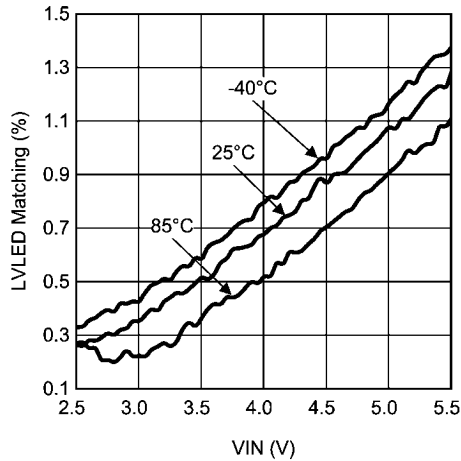
LVLED Matching vs VIN, Temp (ILED = 20mA)
