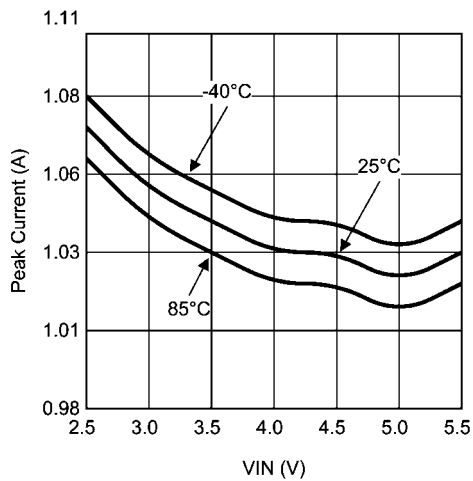
Closed Loop Current Limit vs VIN
