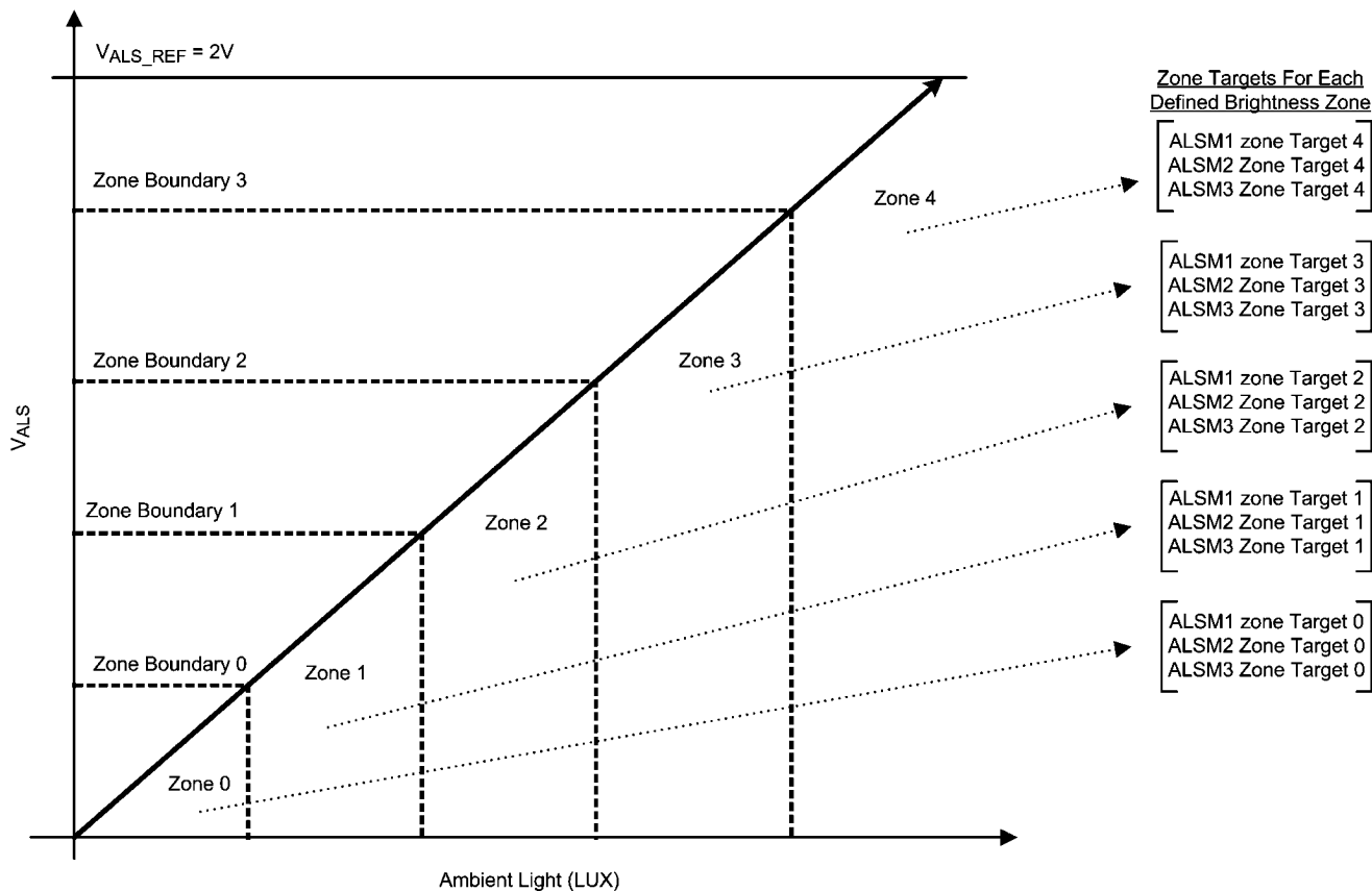
FIGURE 7. ALS Brightness Zone to Backlight Current Mapping
