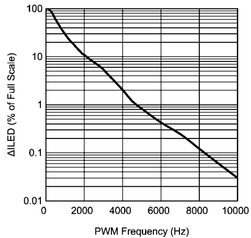
LED Current Ripple vs f_{PWM} (50% Duty Cycle, I_{LED\_FULL\_SCALE} = 20.2mA )
