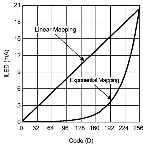
FIGURE 5. LED Current Mapping Modes
