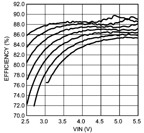
Efficiency vs VIN, Dual String L = 10 \mu H, 20mA/string, f SW = 1MHz Top to Bottom: 2x4, 2x5, 2x6, 2x7, 2x8, 2x9, 2x10 (LEDs)
