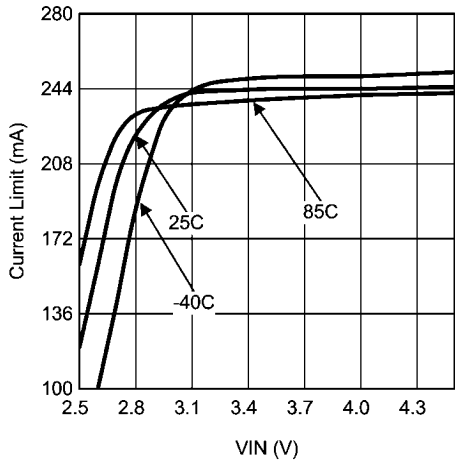
Charge Pump Short Circuit Current Limit vs VIN (2X Gain)
