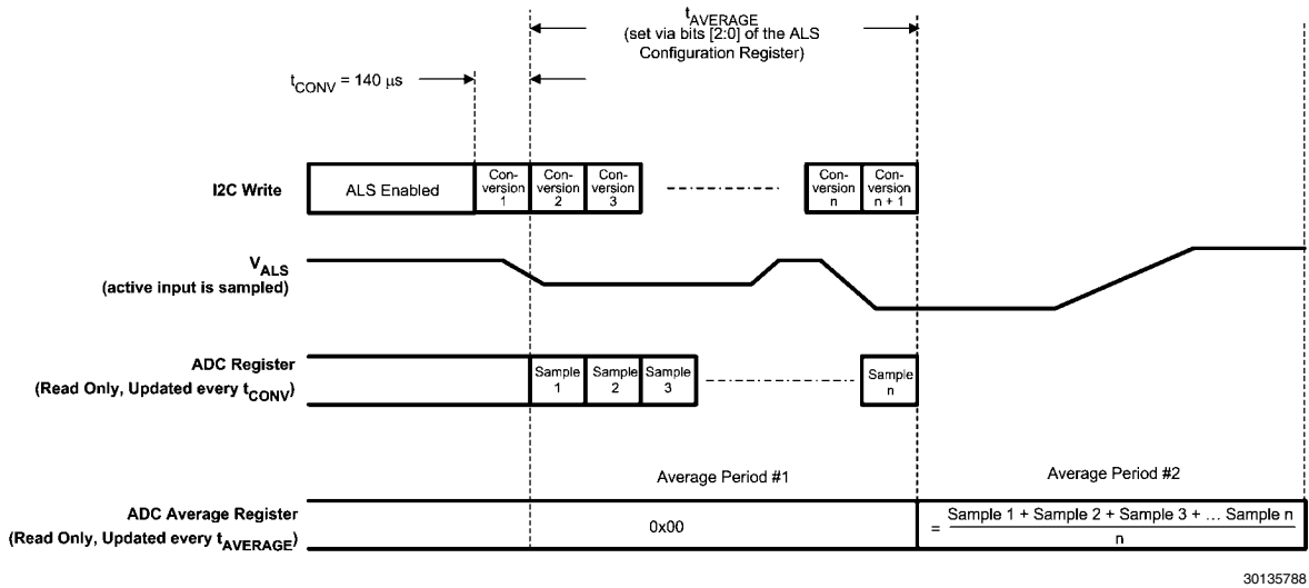
FIGURE 9. ADC Timing
