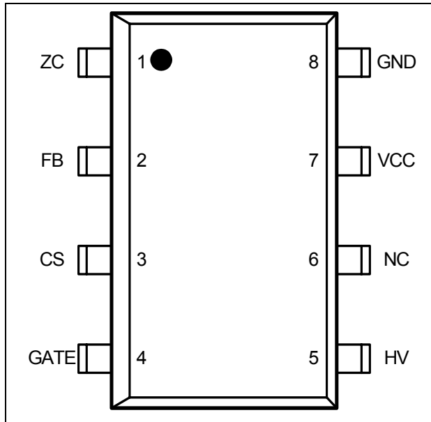
Figure 1 Pin Configuration PG-DSO-8(top view)
