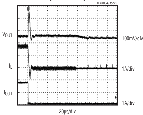
LOAD TRANSIENT RESPONSE (1.8A to 5mA)
