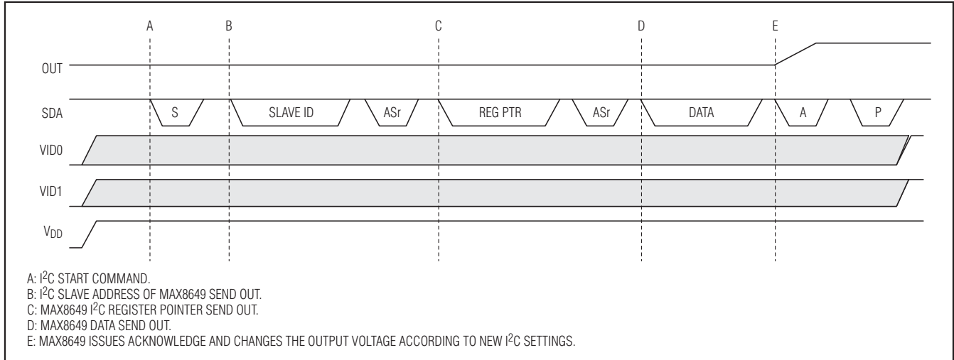
Figure 13. Update Output Operation
